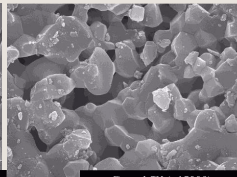
Genesis™ (x15000)
