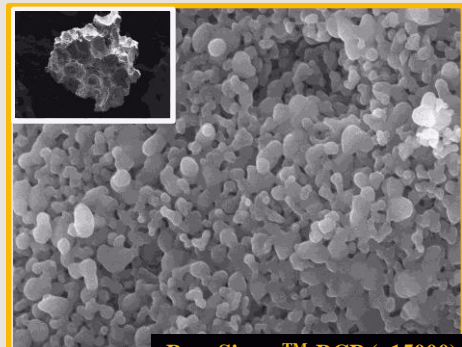
BoneSigma™-BCP (x15000)
