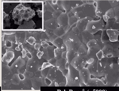
PolyBone® (x5000)
